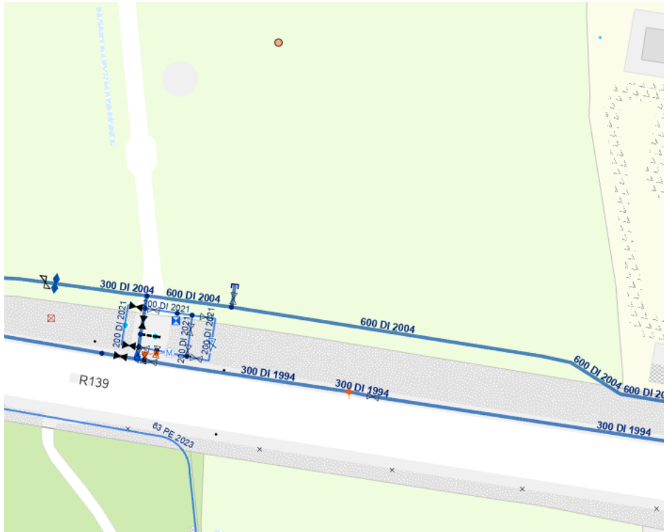
Figure 1 – Existing Uisce Éireann water mains at the site entrance
